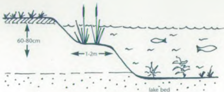
Figure 2: Bankside berm
