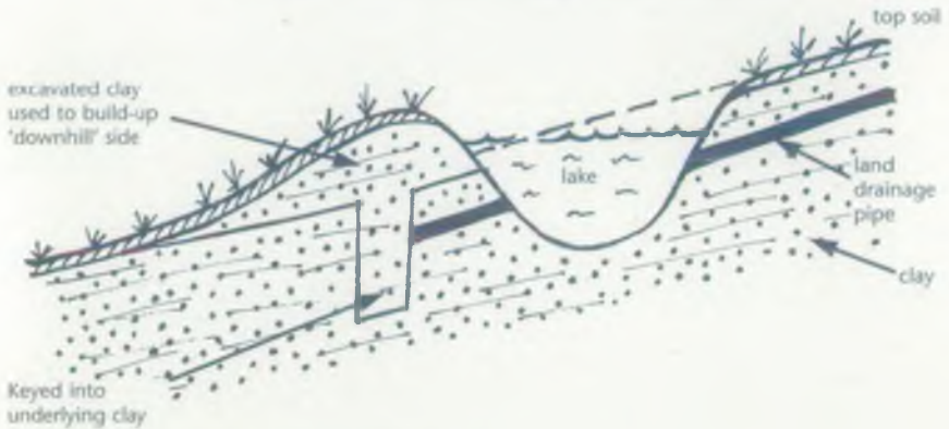
Figure 3: 'Cut-and-fill'
